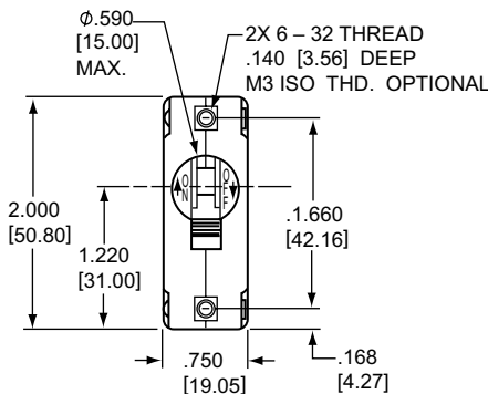
Single Pole Mounting Detail
