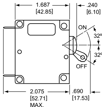
Single Pole Protector
